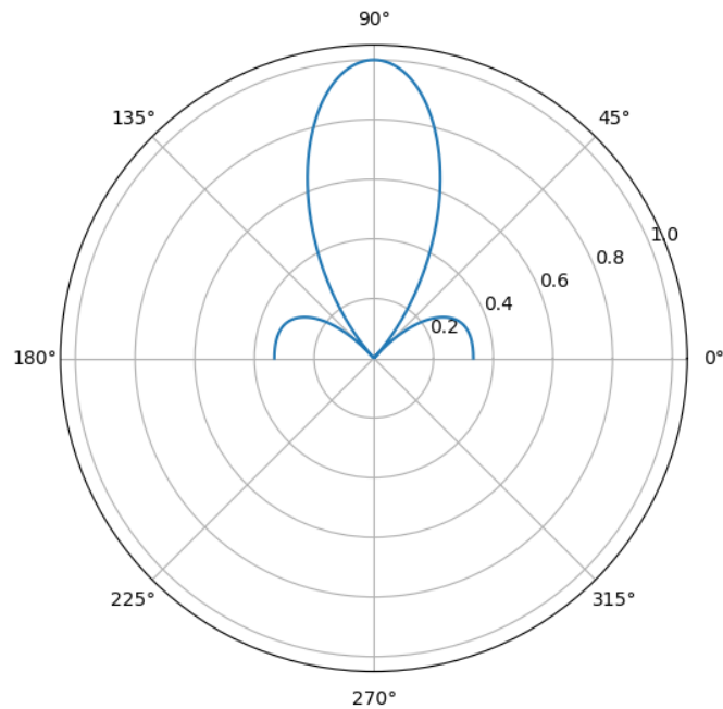
Figure 5: 2D Radiation Pattern of 3-Element Broadside Array Antenna
