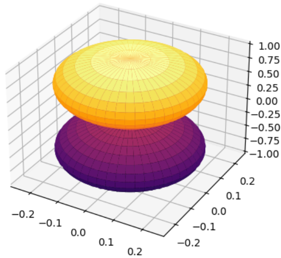
Figure 3: 3D Radiation Patterns of Horn Antenna
