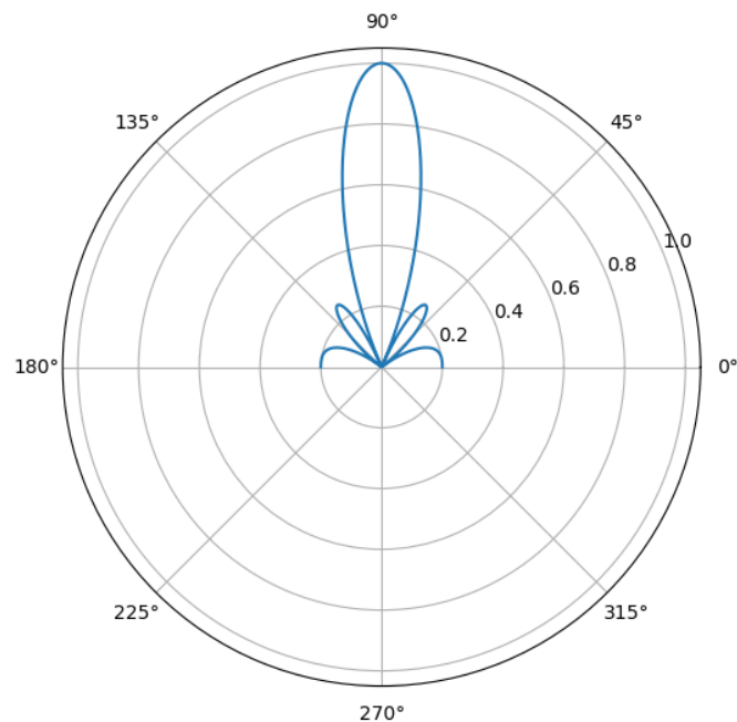
Figure 9: 2D Radiation Pattern of 5-Element Broadside Array Antenna
