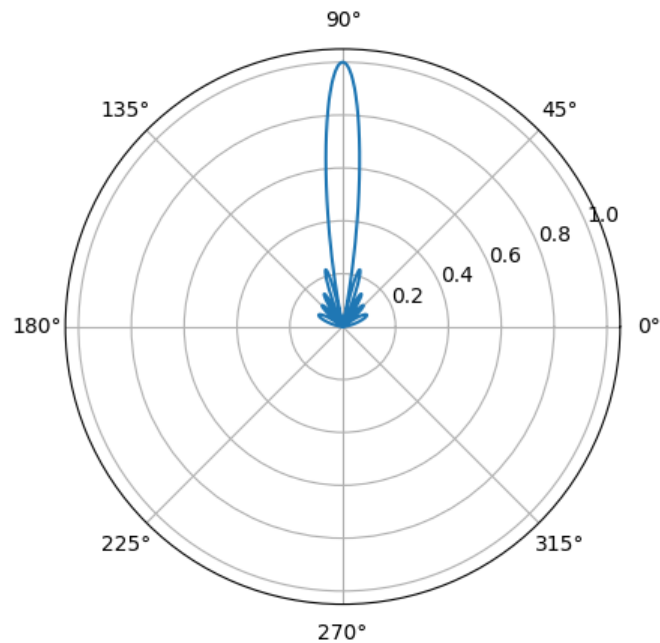
Figure 4: 2D Radiation Pattern of Linear Antenna Array
