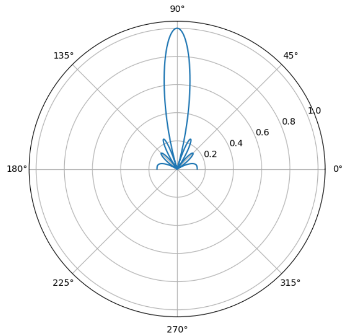
Figure 10: 2D Radiation Pattern of 7-Element Broadside Array Antenna
