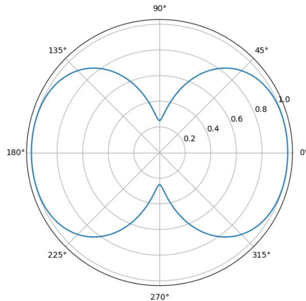
Figure 8: Far-Field Radiation Pattern (Unequal Amplitude and Opposite Phase)
