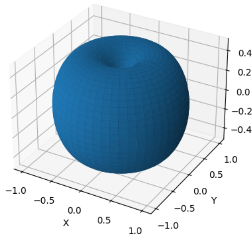
Figure 1: 3D Radiation Patterns of Dipole Antenna
