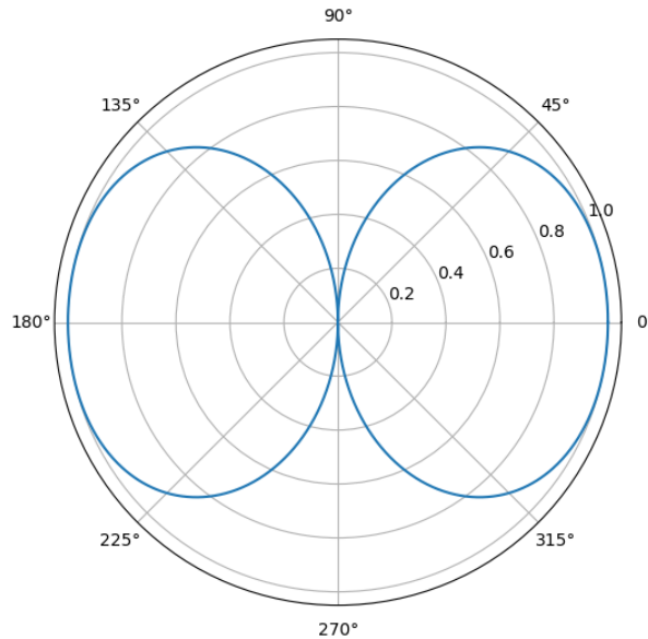
Figure 7: Far-Field Radiation Pattern of Two Isotropic Sources (Opposite Phase)
