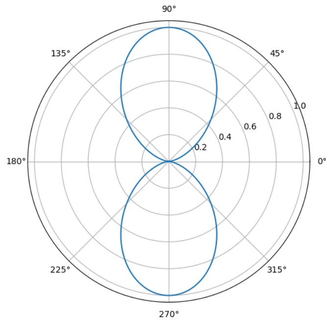
Figure 6: Far-Field Radiation Pattern of Two Isotropic Point Sources
